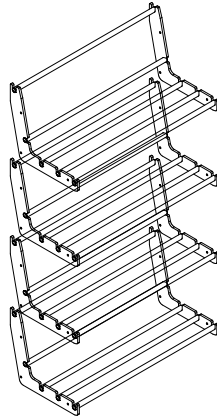
KIT 4 RIPIANI TUBI INCLINATI KIT 4 INCLINED TUBE SHELVES
